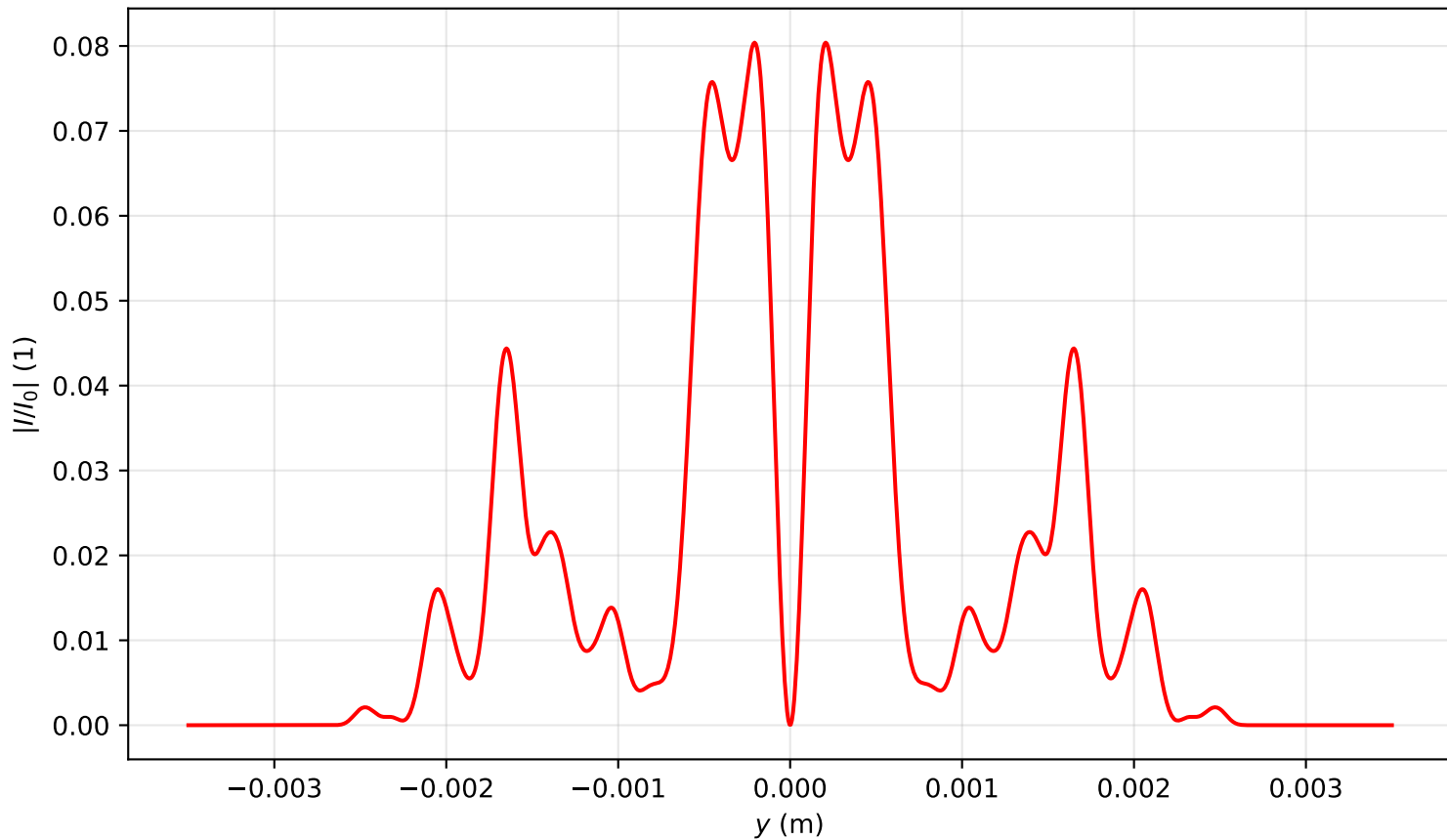
Intensity profile I(x = 0, y, z = 2.786)/I_0 , P_{in}=8.0P_{cr} , artificial time
